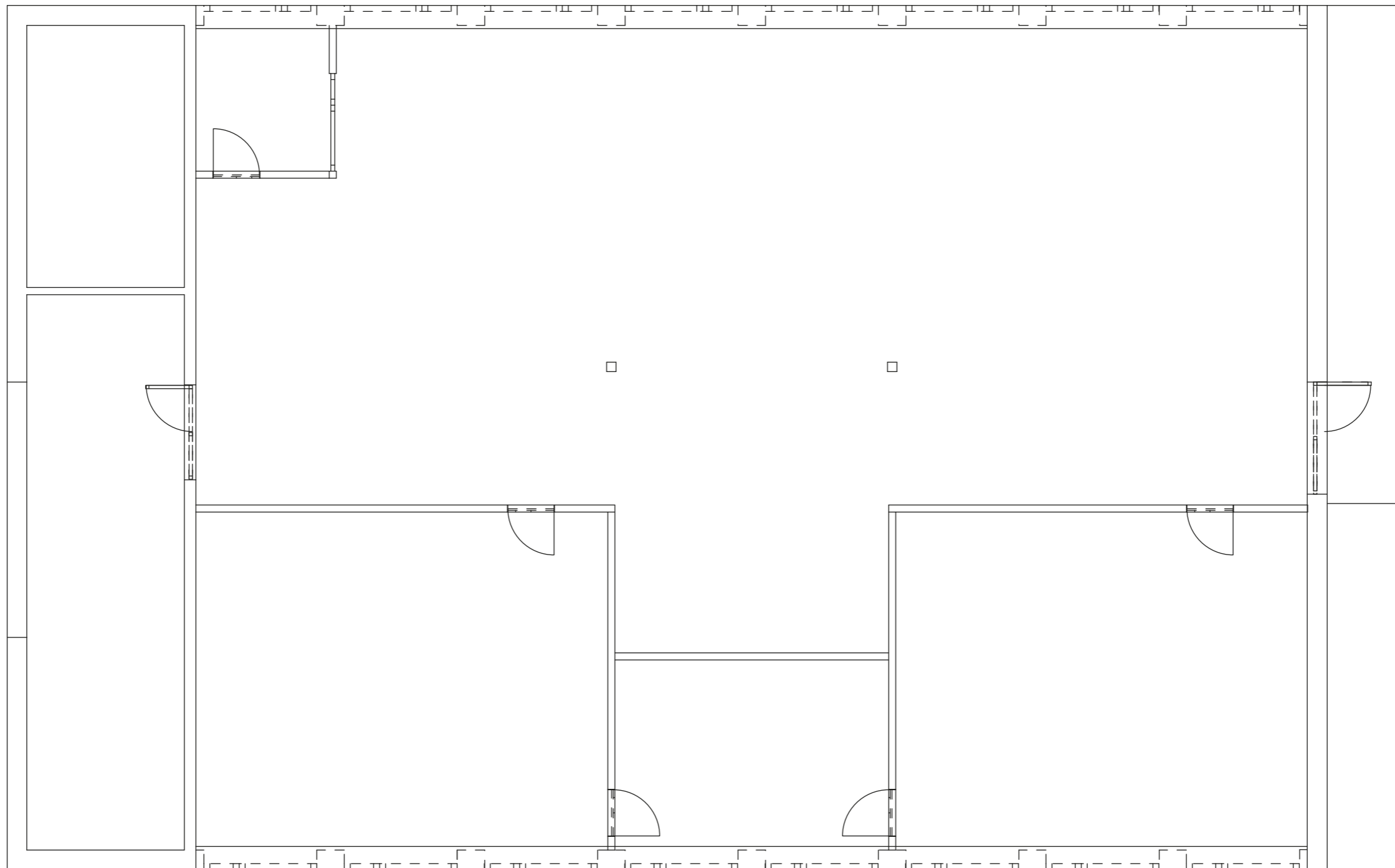
Raumkonzept Praxis | IN-BETWEEN | Maßstab 1:100 (DIN A3)
